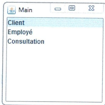
Figure 5.21 : Class main
